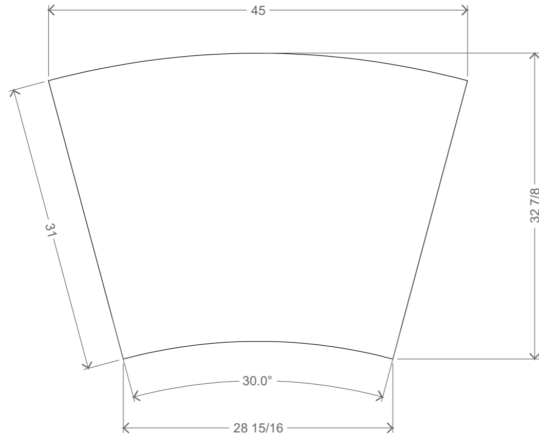
FRONT VIEW
